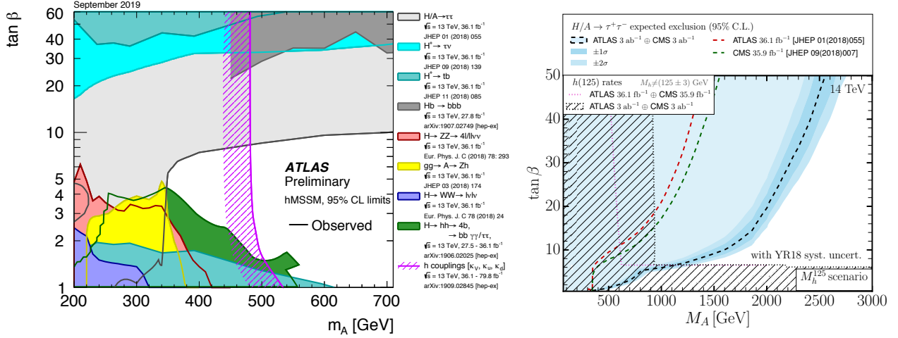
Figure 11.19: The 95% CL exclusion contours in the (M_A, \tan \beta) parameter space for: (left) a summary of ATLAS Run 2 searches in the hMSSM and (right) the projected sensitivity for the combination of ATLAS and CMS searches in the A, H \rightarrow \tau^+\tau^- channel at HL-LHC and the interpretation of the constraints from the measurements of the Higgs boson couplings in the M_h^{125} benchmark [353] (the projected ATLAS sensitivity in the A, H \rightarrow \tau^+\tau^- channel used for this projection was not optimised for high masses, when re-optimised similar sensitivities are obtained between ATLAS and CMS).
