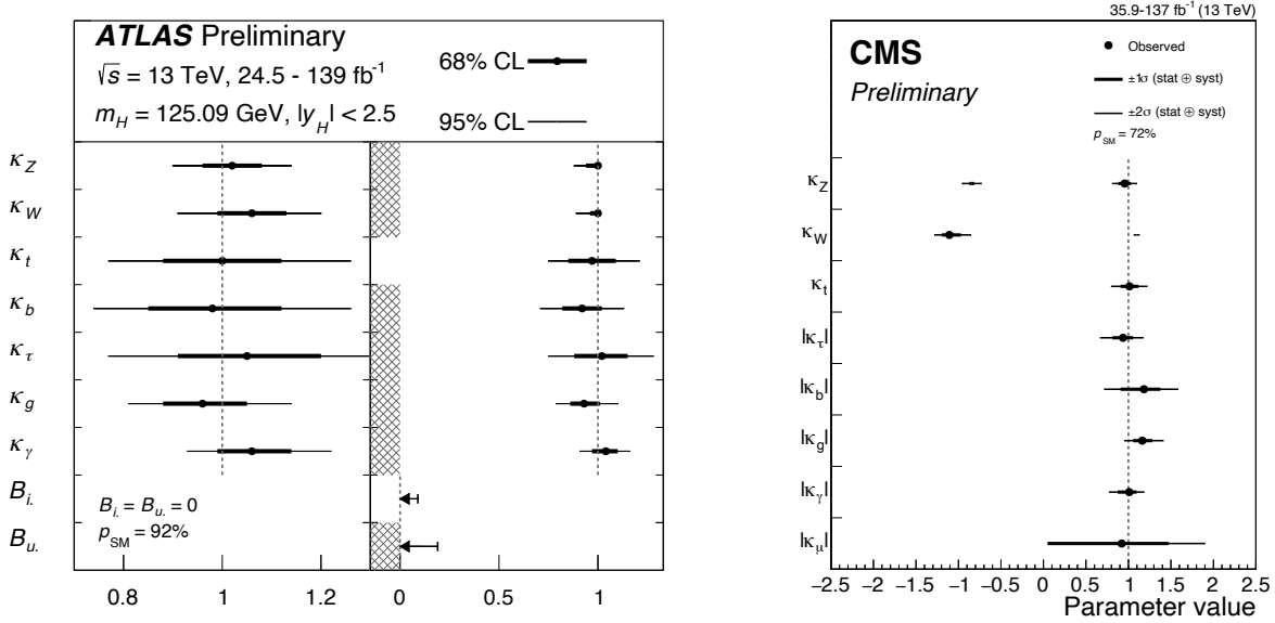
Figure 11.14: ATLAS [241] (left) and CMS [242] (right) combined measurements of coupling modifiers with various assumptions on the \kappa_V < 1 scenario, and in the case of the ATLAS measurements with the assumption \text{BR}_{\text{BSM}} = 0 and using the off-shell Higgs measurements.
