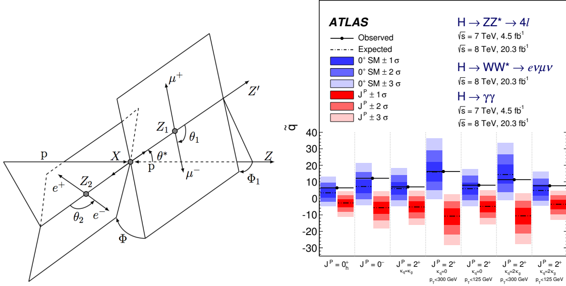
Figure 11.9: (Left) Definition of the production and decay angles defined for the H \rightarrow ZZ^{(*)} \rightarrow 4\ell final state [248]. (Right) Expected distributions of the test statistic for the SM hypothesis (in blue) and several alternative spin and parity hypotheses (in red).
