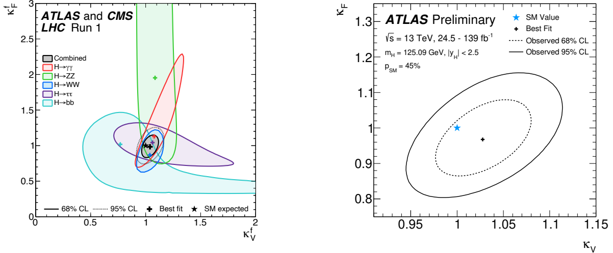
Figure 11.12: Likelihood contours in the (\kappa_F, \kappa_V) plane for the ATLAS-CMS Run1 combination [299] (left) and ATLAS [241] (right) individual Run2 combinations. These results correspond to a 2-parameter fit assuming a universal rescaling of the Higgs couplings to all fermions and also \kappa_W = \kappa_Z .
