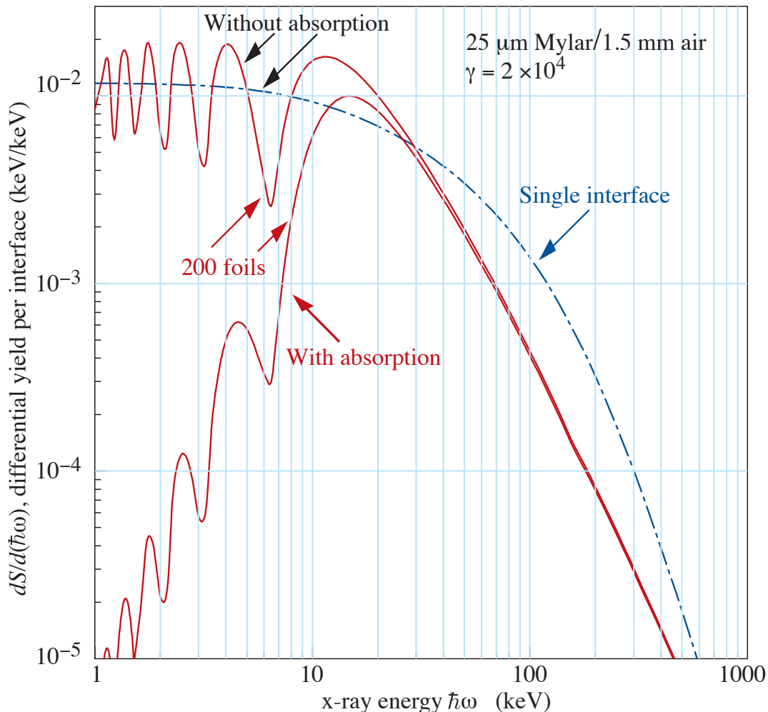
Figure 34.27: X-ray photon energy spectra for a radiator consisting of 200 25\ \mu\text{m} thick foils of Mylar with 1.5\ \text{mm} spacing in air (solid lines) and for a single surface (dashed line). Curves are shown with and without absorption. Adapted from Ref. [89].
